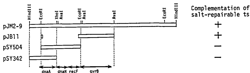
Fig. 1. Chromosome region that complements the salt-repairable ts mutation. The 13 kb Hind III fragment containing dnaA-gyrB region or part of this fragment was carried by the plasmids as shown with rectangles. Complementation was examined with W3110 parA110 . The plasmids were generous gifts from Drs. J. Yamagishi and S. Yasuda, to whom we are obliged.
