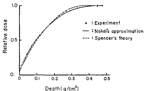
Fig. 1. Comparison of the depth dose curve of polystyrene for ^{60}\text{Co} \gamma -ray with the theoretical curve.
