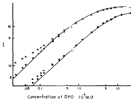
Fig. 1. Comparison of theoretical curves of fluorescence intensity vs. solute concentration with experimental values for the aerated DPO-toluene solutions excited by 260 m\mu UV. Curves A and B are calculated ones, ( \Delta ) and ( \blacktriangle ) are the observed values for \text{CCl}_4 concentration of zero and 1.7 \times 10^{-3} M/l , respectively.
