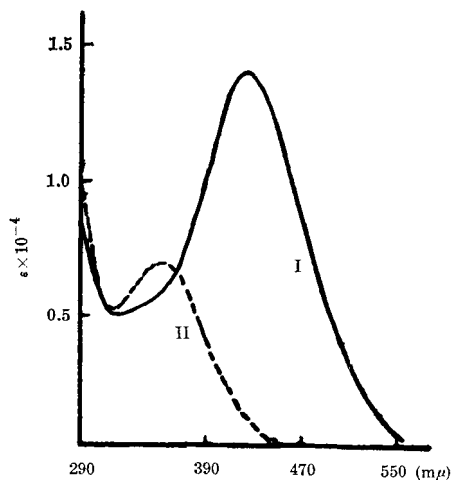
Fig. 1. Absorption spectra of TNP-DNA. Curve I, at pH 10; Curve II, at pH 3.
