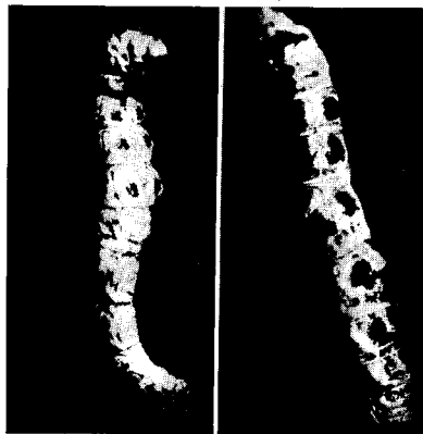
Fig. 1. Larvae homozygous for E^{rc} . A: abdominal view B: dorsal view
